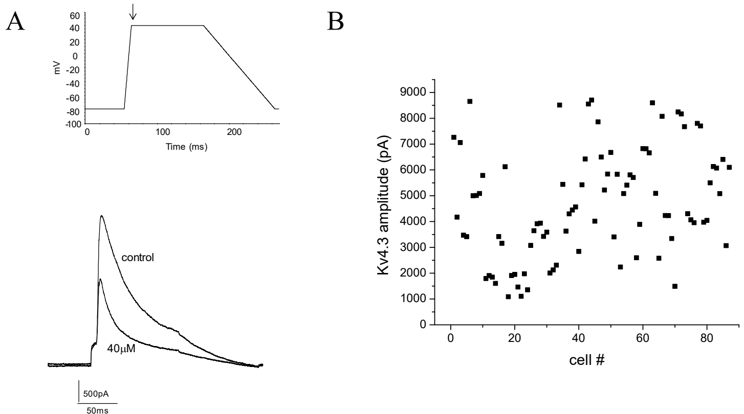
Figure: A. Recording of Kv4.3 current in the absence and presence of quinine. B. Current amplitude plot taken from 87 cells. All recordings were performed at 22°C using manual patch clamp.
